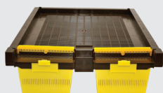
Pollen Collector Set For ANEL Bottom Boards
