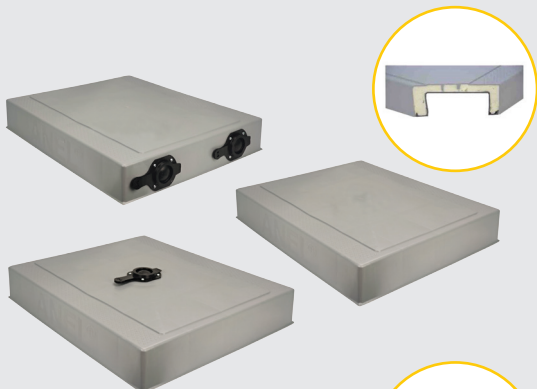
Beehive Top Cover ANEL With or Without Ventilations / Entrances Langstroth With PU Insulation
