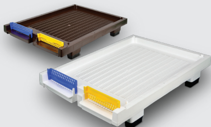
Beehive Bottom Board ANEL Hybrid Ventilated (Anti-Varroa) or Closed Langstroth With Conversion to Pollen Collector
